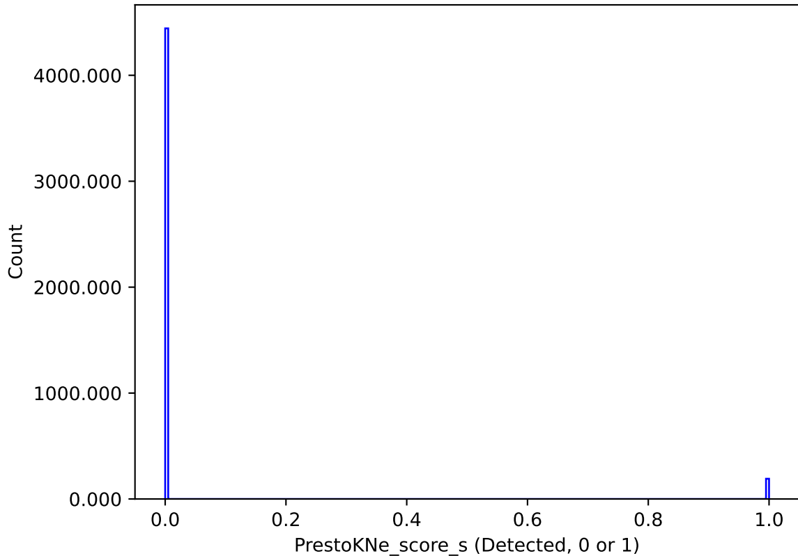
too_5_1v3.4_10yrs : PrestoKNe_score_s
