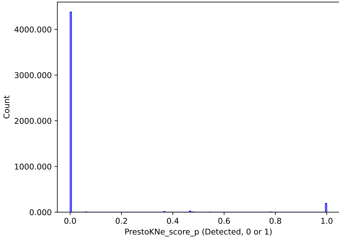
too_5_1v3.4_10yrs : PrestoKNe_score_p
