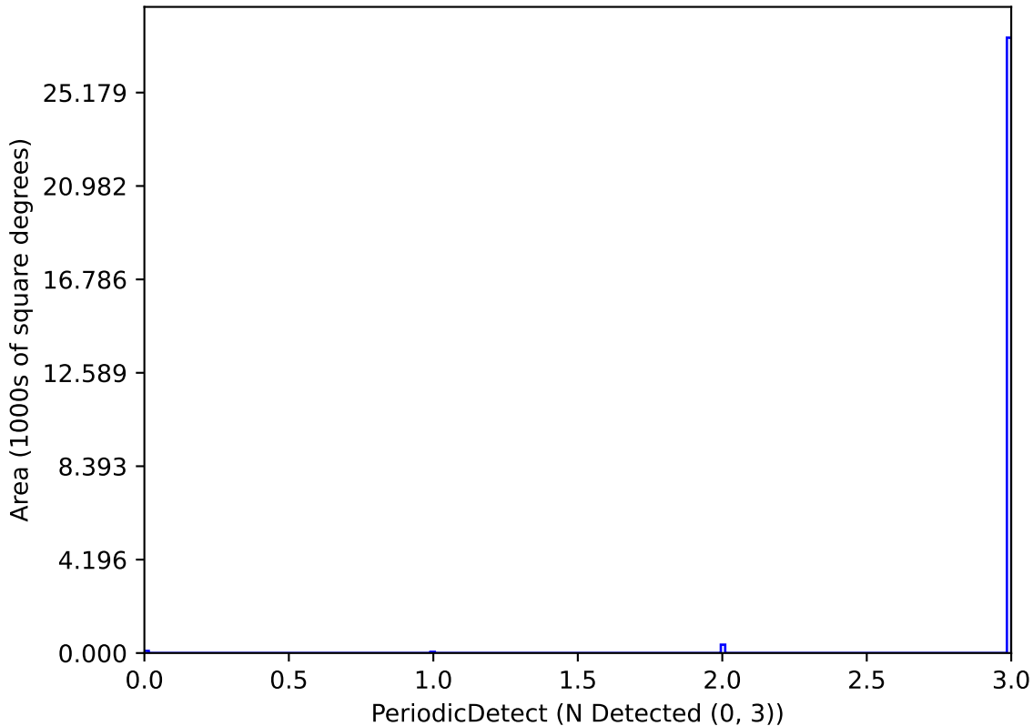
too_5_1v3.4_10yrs P_2.0_Mag_21_Amp_0.05-0.1-1: PeriodicDetect
