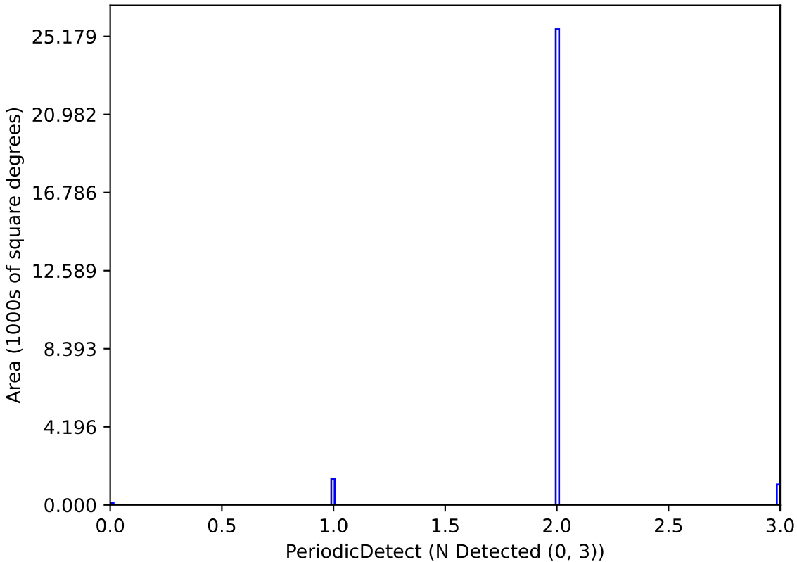
too_5_1v3.4_10yrs P_1.0_Mag_21_Amp_0.05-0.1-1: PeriodicDetect
