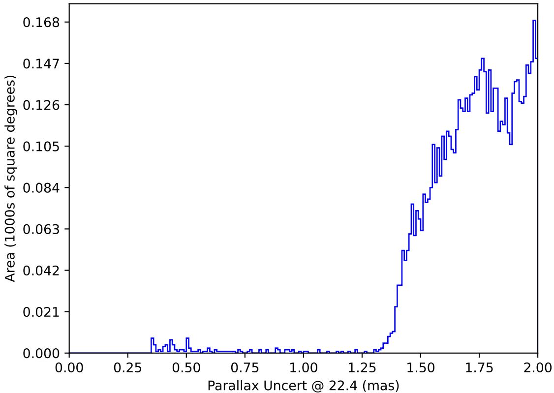
too_5_1v3.4_10yrs : Parallax Uncert @ 22.4
