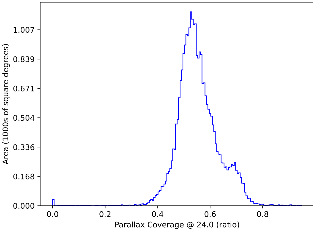
too_5_1v3.4_10yrs : Parallax Coverage @ 24.0
