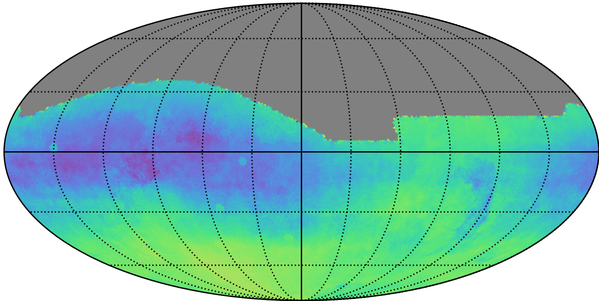
too_5_1v3.4_10yrs : Parallax-DCR degeneracy @ 24.0
