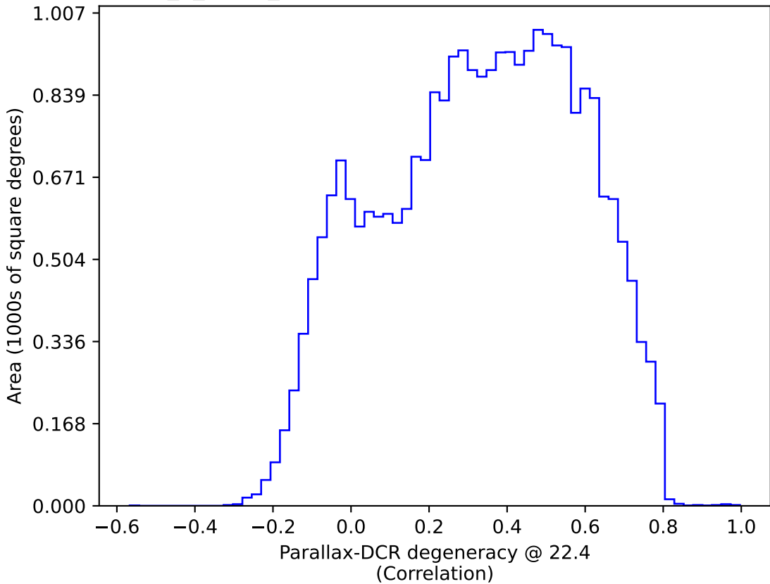
too_5_1v3.4_10yrs : Parallax-DCR degeneracy @ 22.4
