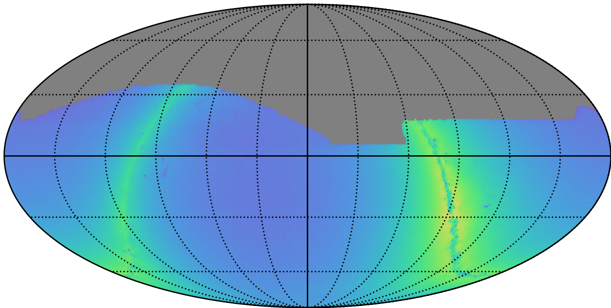
too_5_1v3.4_10yrs z: Nstars_no_crowding
