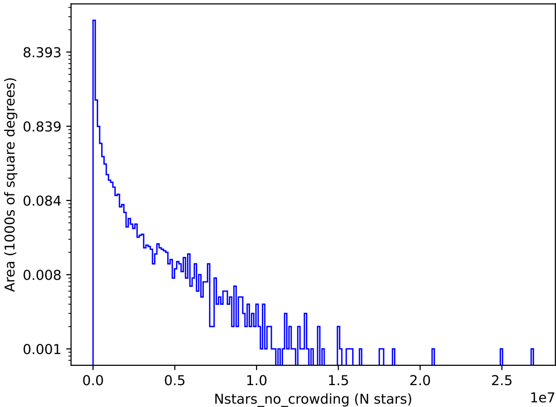
too_5_1v3.4_10yrs z: Nstars_no_crowding
