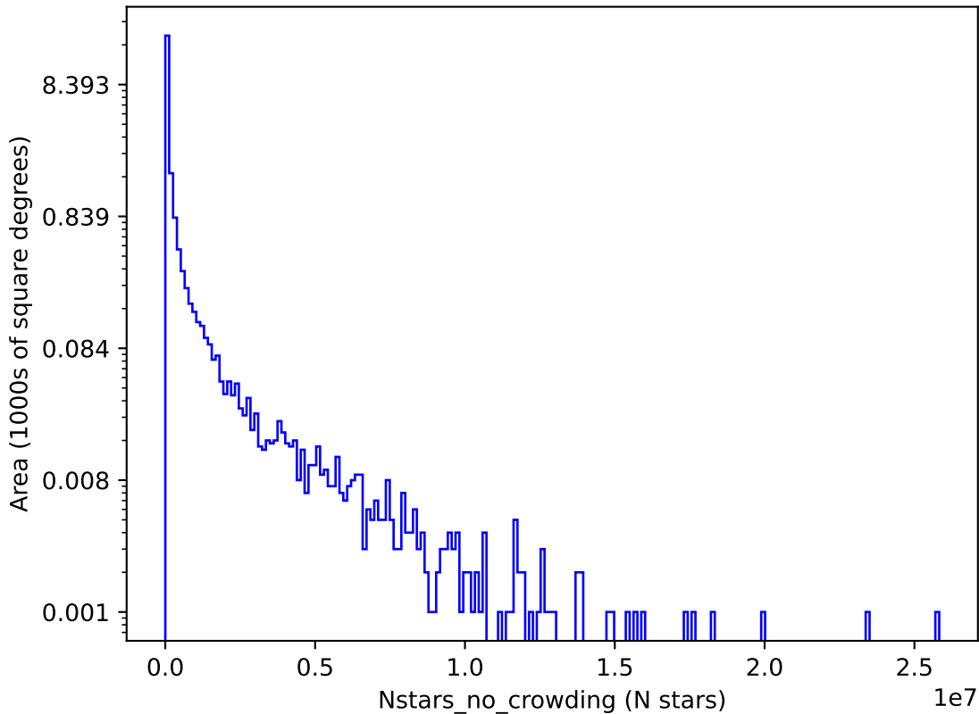
too_5_1v3.4_10yrs y: Nstars_no_crowding
