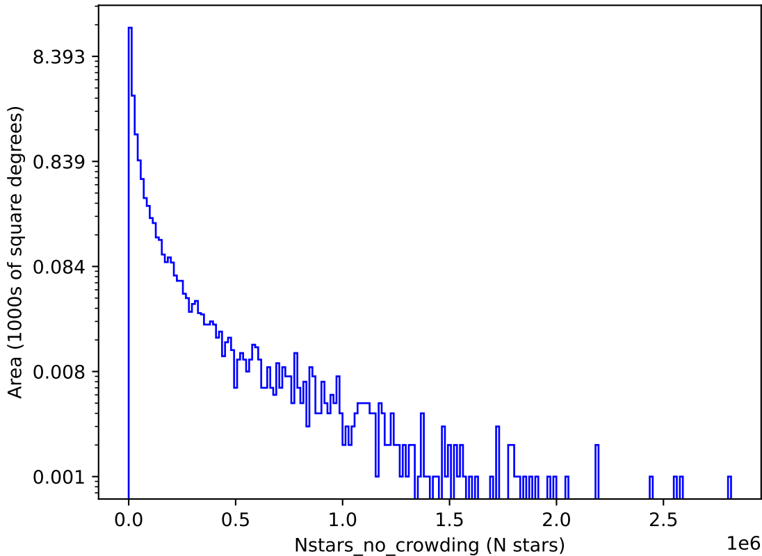
too_5_1v3.4_10yrs u: Nstars_no_crowding
