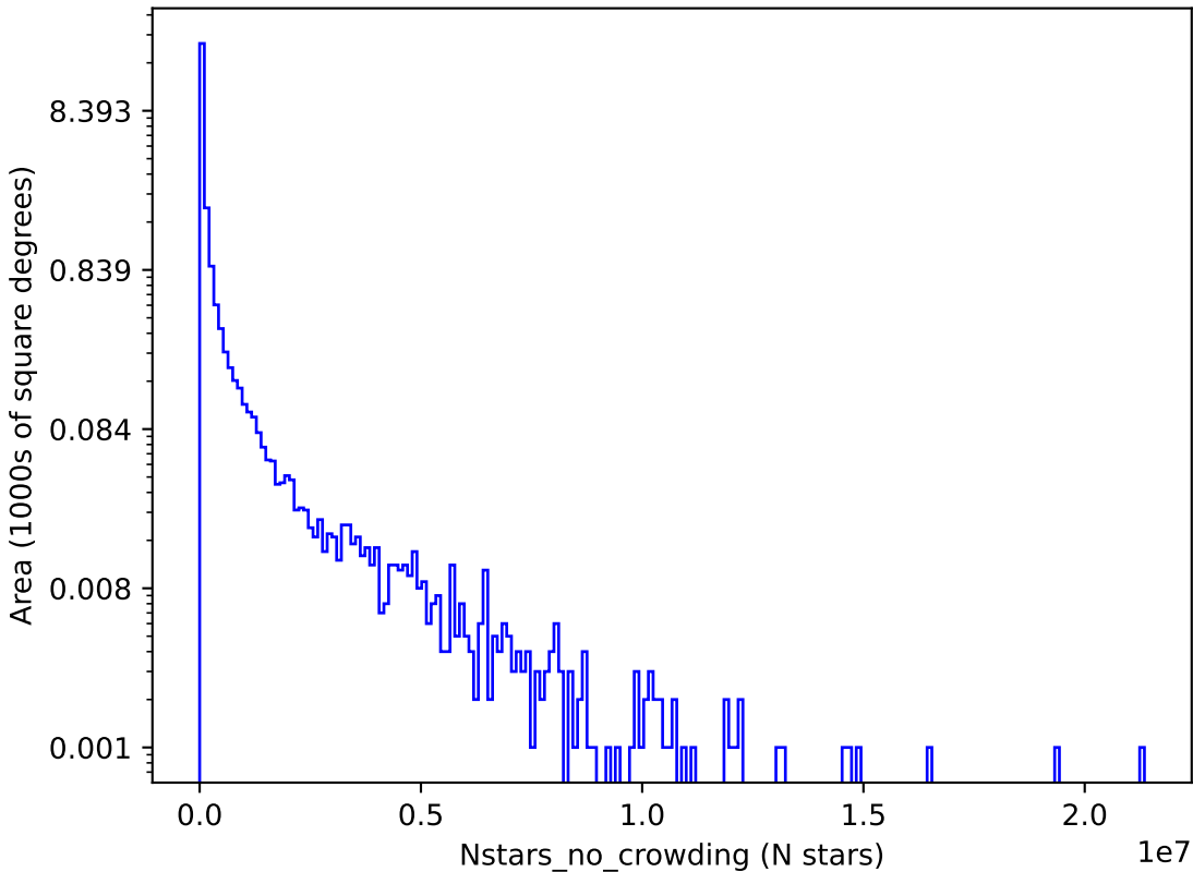
too_5_1v3.4_10yrs r: Nstars_no_crowding
