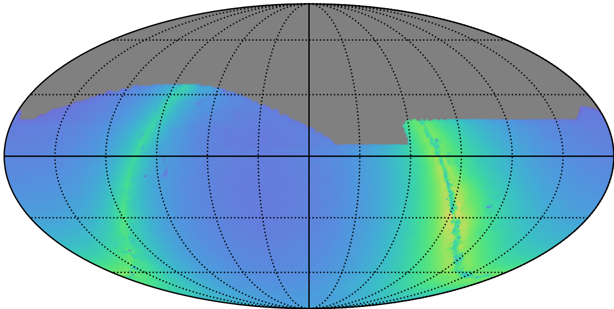
too_5_1v3.4_10yrs i: Nstars_no_crowding
