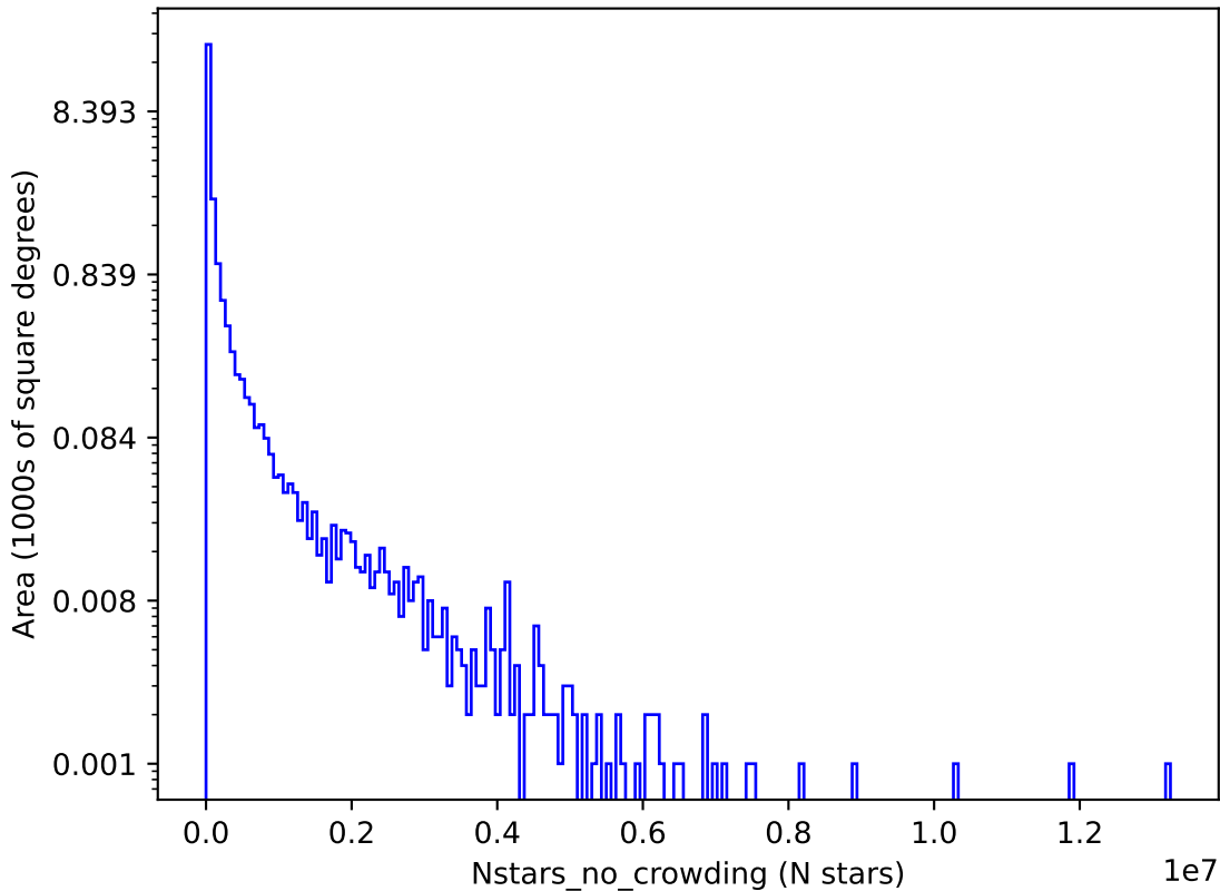
too_5_1v3.4_10yrs g: Nstars_no_crowding
