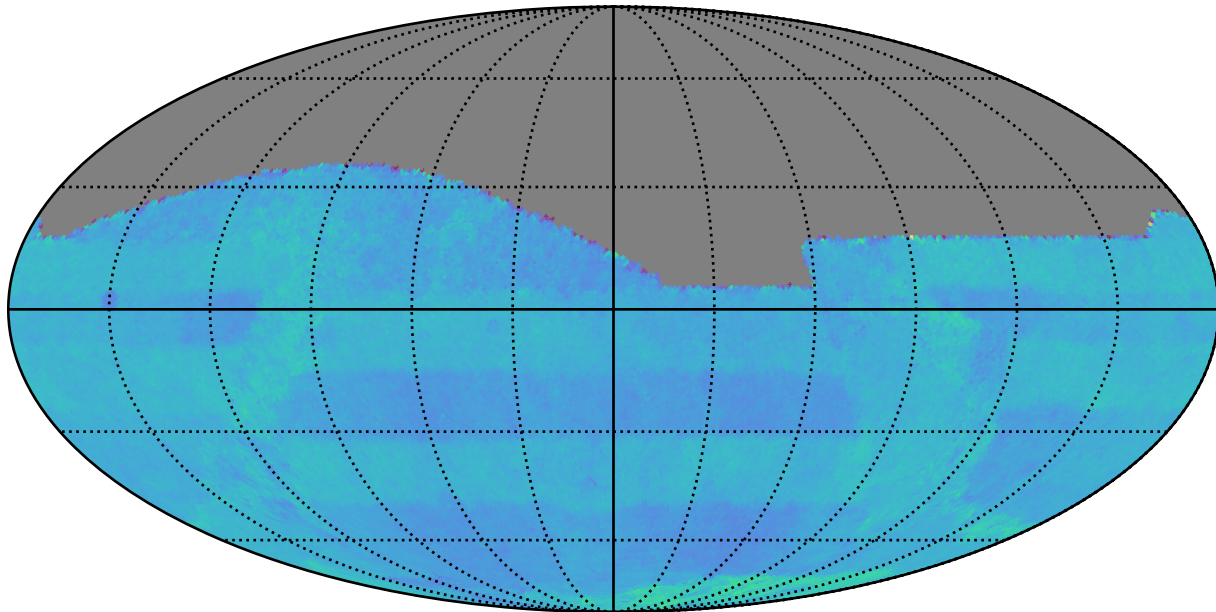
too_5_1v3.4_10yrs : Normalized Proper Motion Uncert @ 24.0
