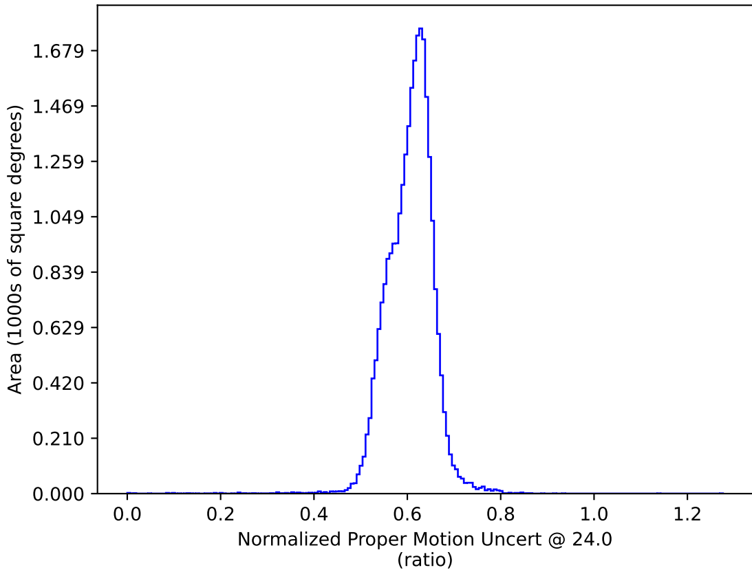
too_5_1v3.4_10yrs : Normalized Proper Motion Uncert @ 24.0
