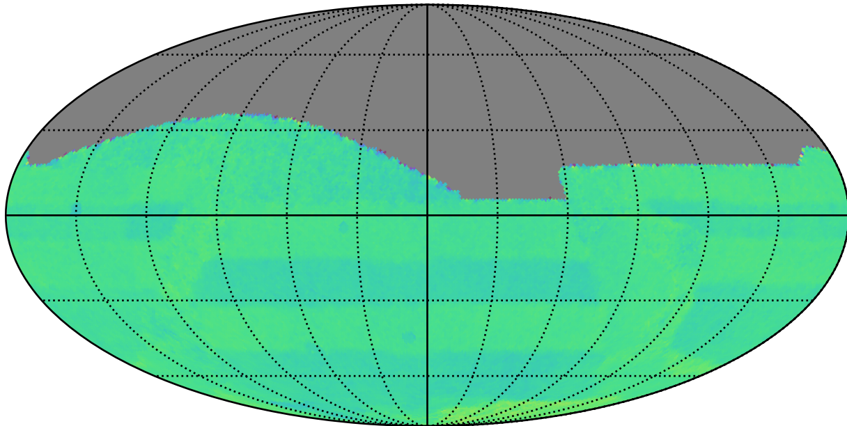
too_5_1v3.4_10yrs : Normalized Proper Motion Uncert @ 20.5
