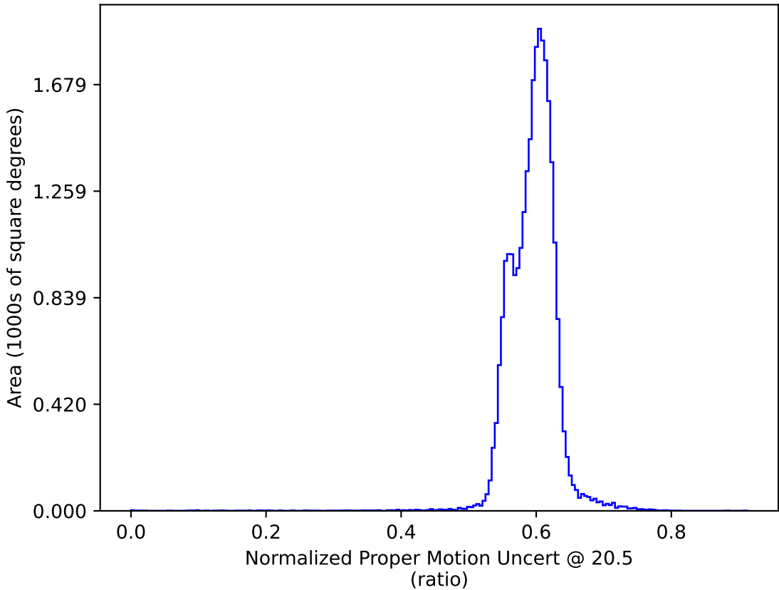
too_5_1v3.4_10yrs : Normalized Proper Motion Uncert @ 20.5
