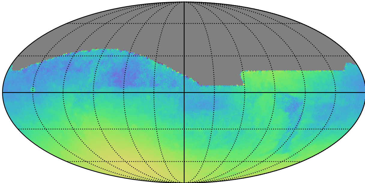
too_5_1v3.4_10yrs : Normalized Parallax Uncert @ 24.0
