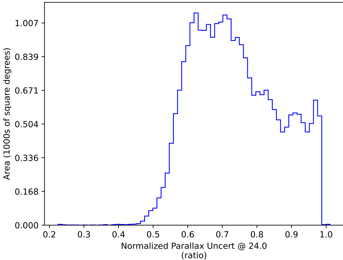
too_5_1v3.4_10yrs : Normalized Parallax Uncert @ 24.0
