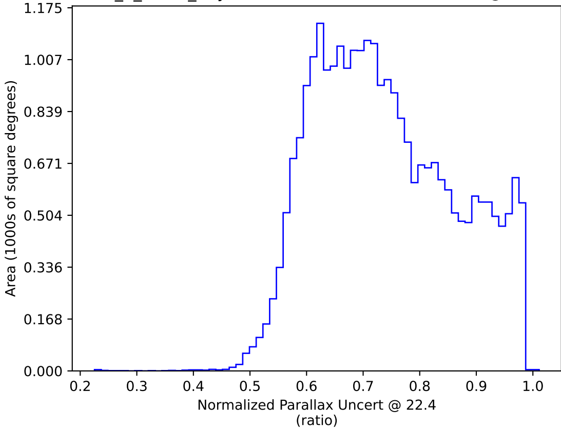
too_5_1v3.4_10yrs : Normalized Parallax Uncert @ 22.4
