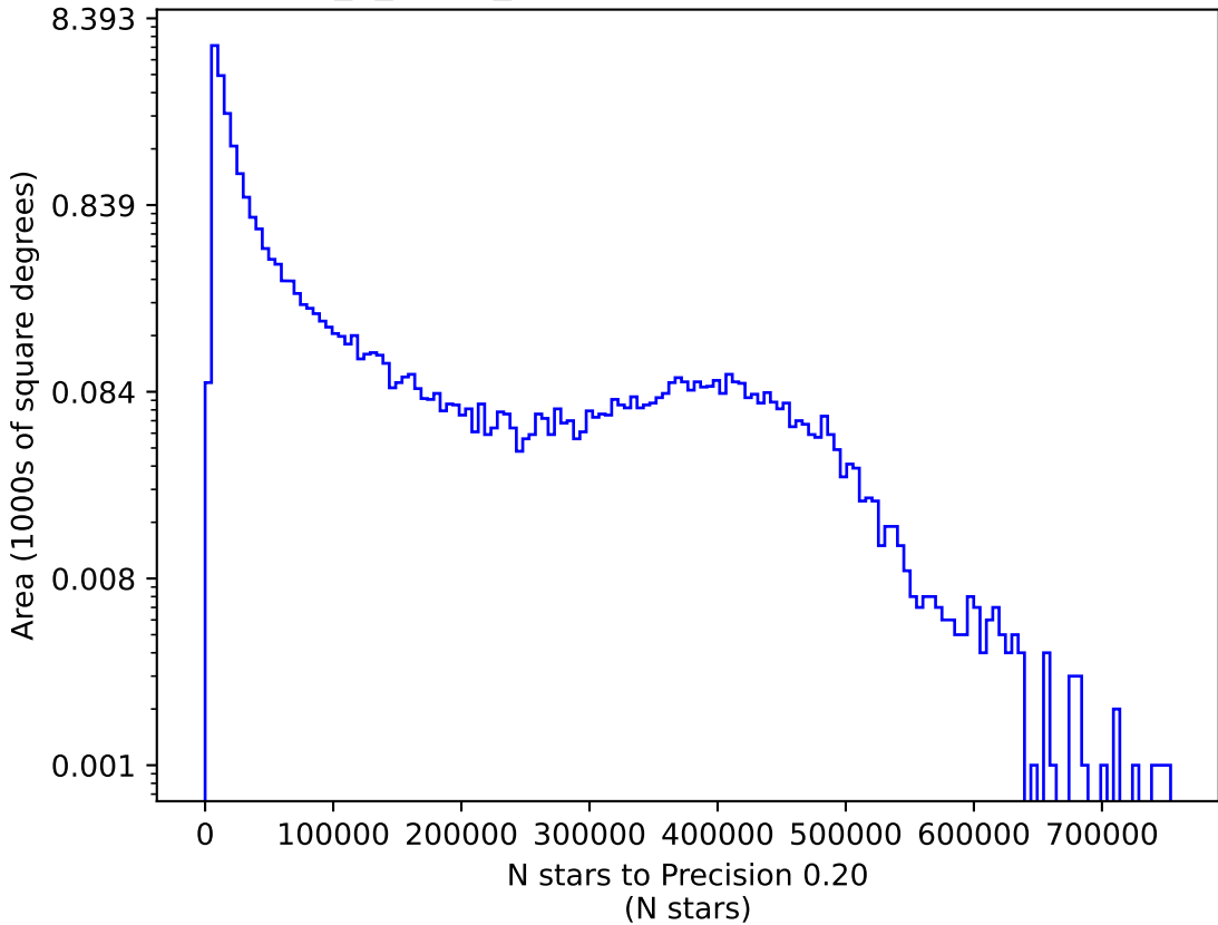
too_5_1v3.4_10yrs z: N stars to Precision 0.20
