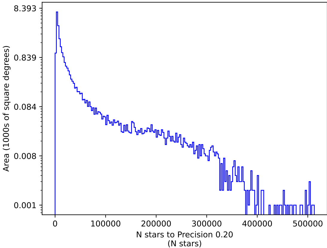
too_5_1v3.4_10yrs u: N stars to Precision 0.20
