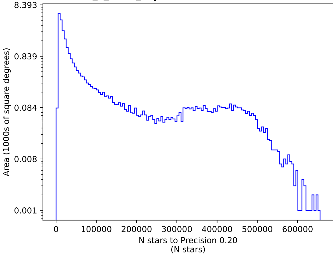
too_5_1v3.4_10yrs i: N stars to Precision 0.20
