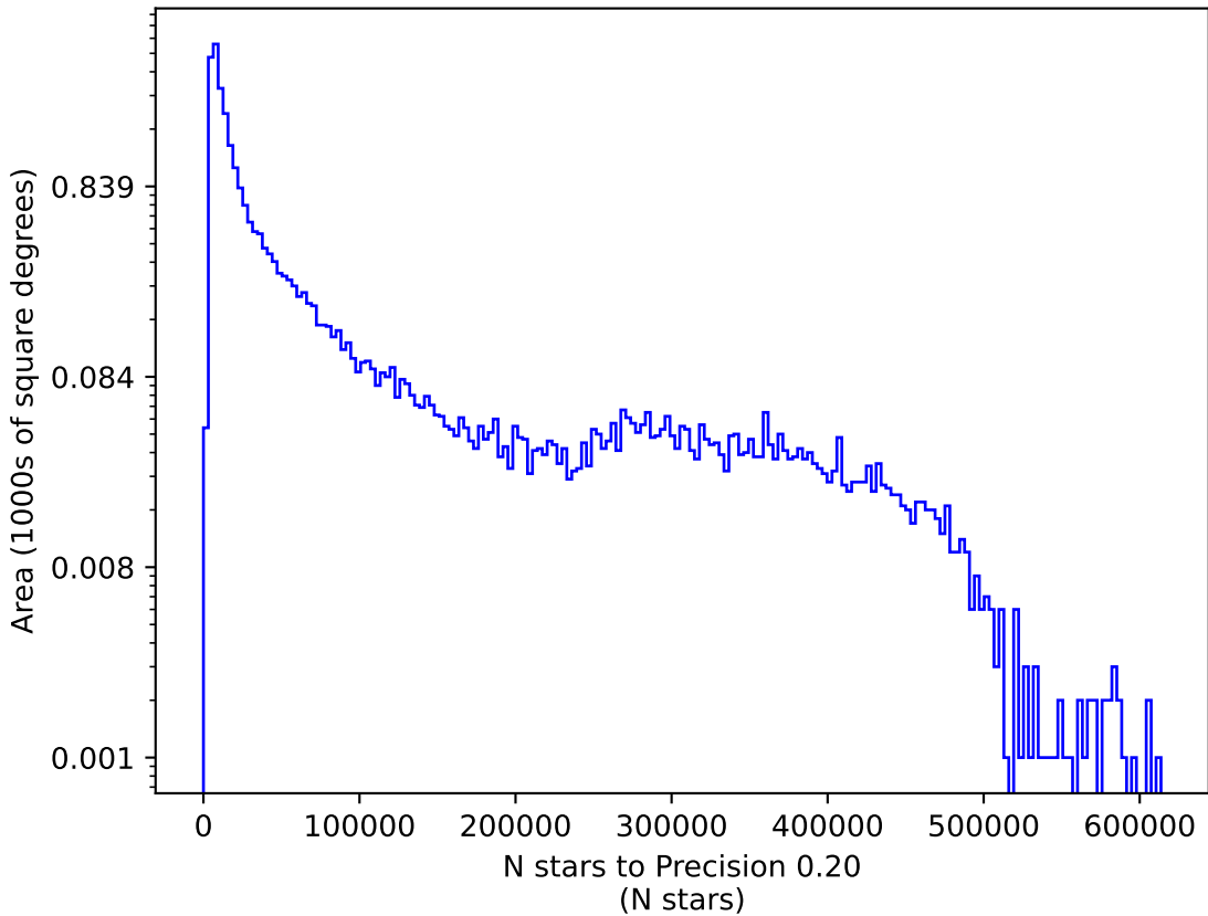
too_5_1v3.4_10yrs g: N stars to Precision 0.20
