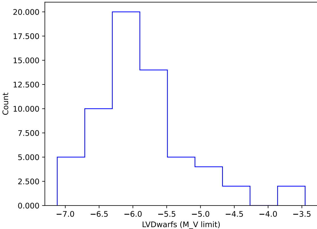
too_5_1v3.4_10yrs gi: LVDwarfs
