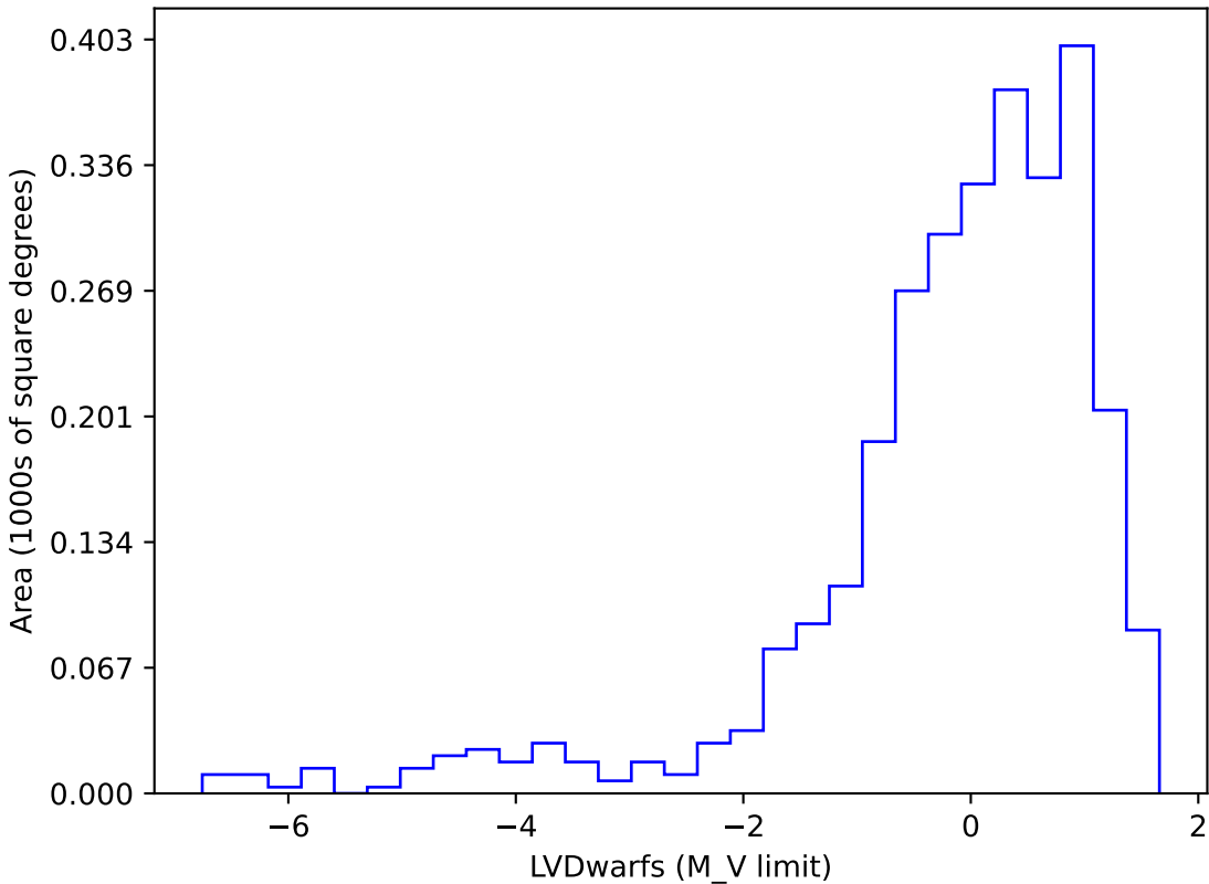
too_5_1v3.4_10yrs gi SCP: LVDwarfs
