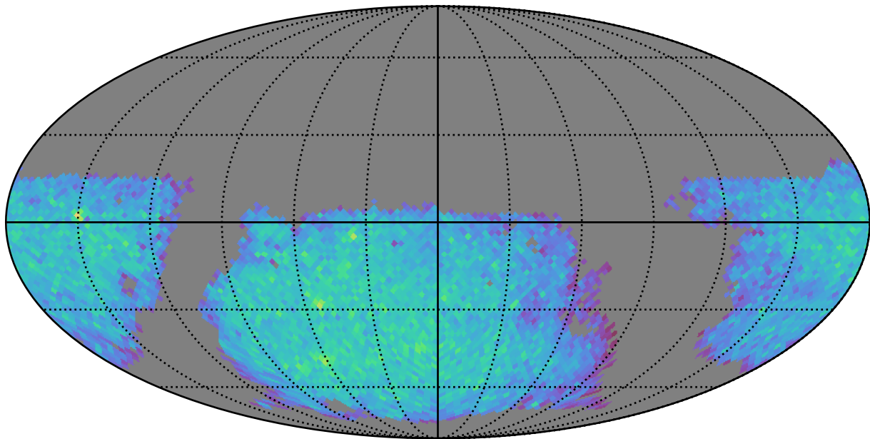
too_5_1v3.4_10yrs gi: LVDwarfs
