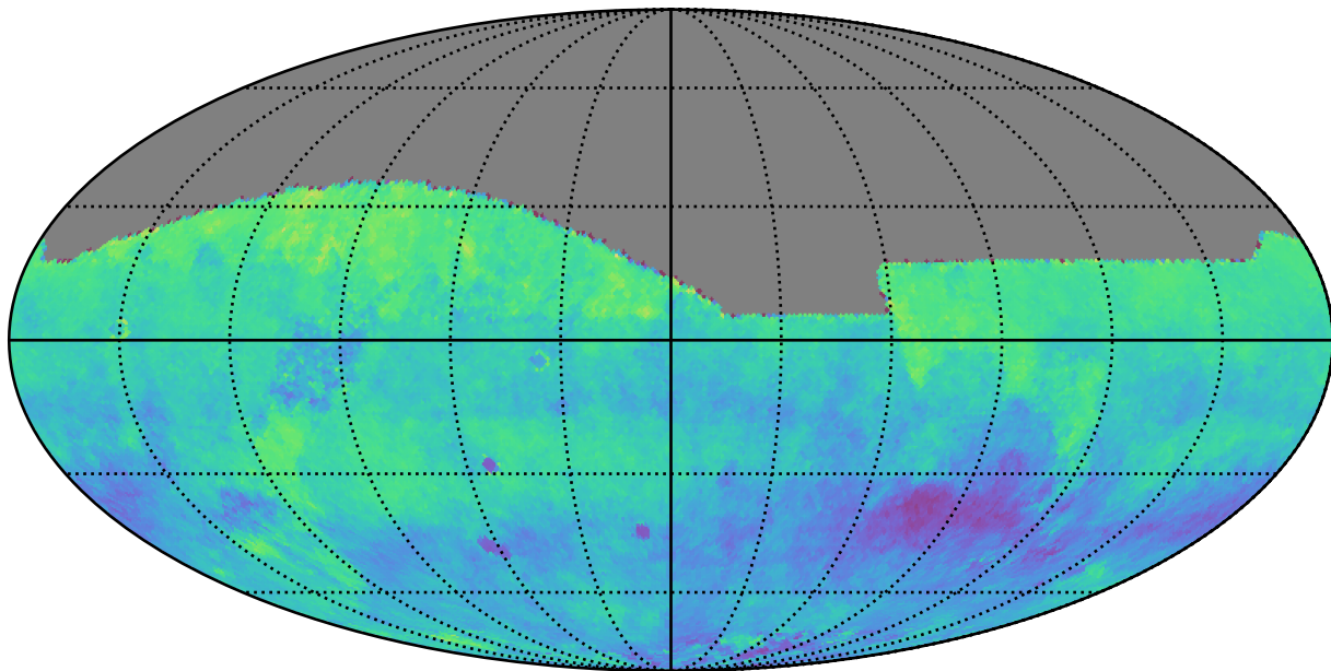
too_5_1v3.4_10yrs z: Kuiper rotSkyPos
