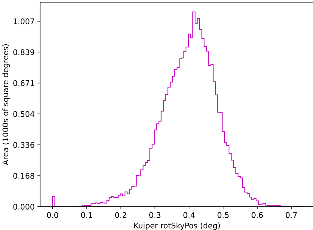
too_5_1v3.4_10yrs z: Kuiper rotSkyPos
