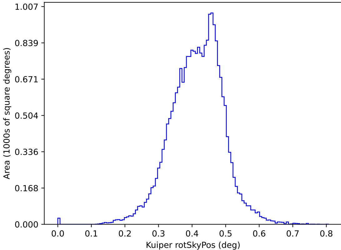
too_5_1v3.4_10yrs y: Kuiper rotSkyPos
