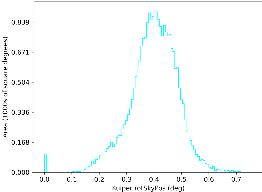
too_5_1v3.4_10yrs u: Kuiper rotSkyPos
