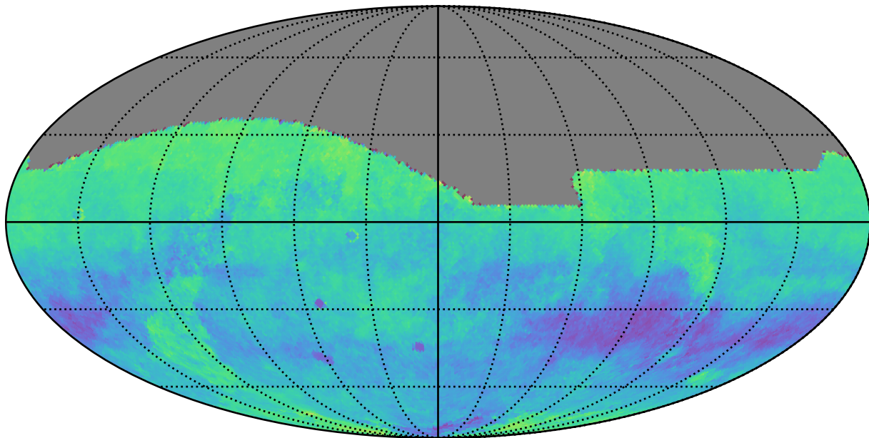
too_5_1v3.4_10yrs r: Kuiper rotSkyPos
