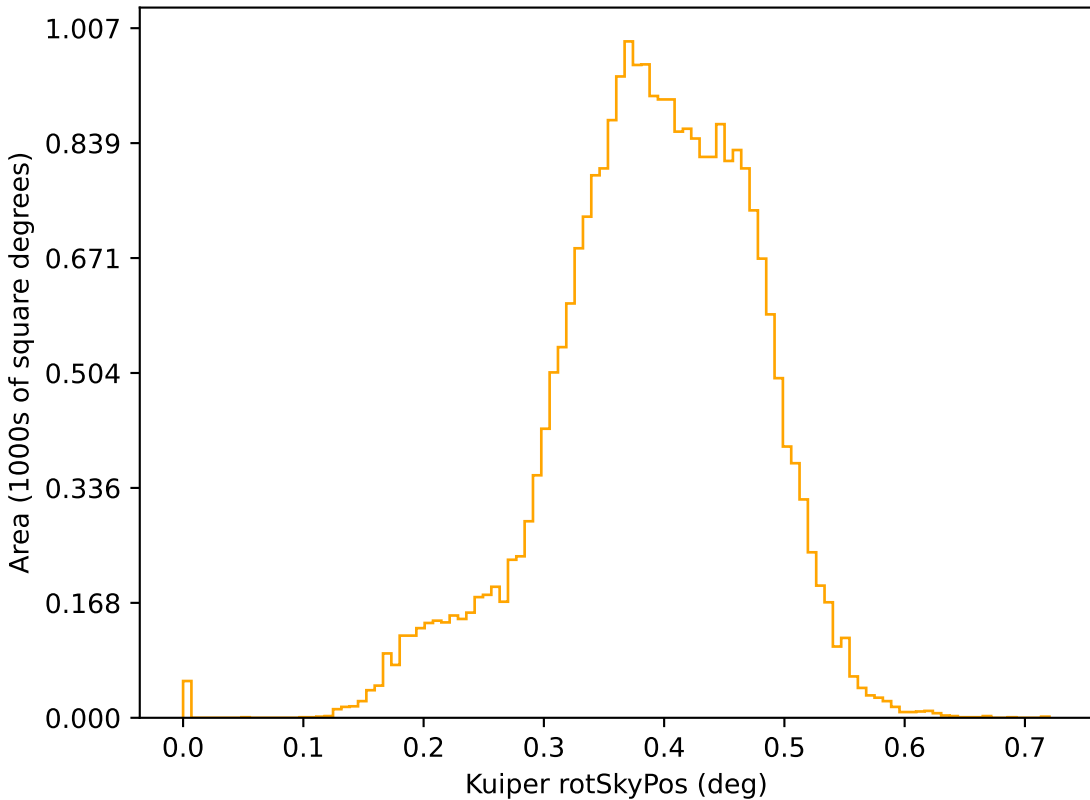
too_5_1v3.4_10yrs r: Kuiper rotSkyPos
