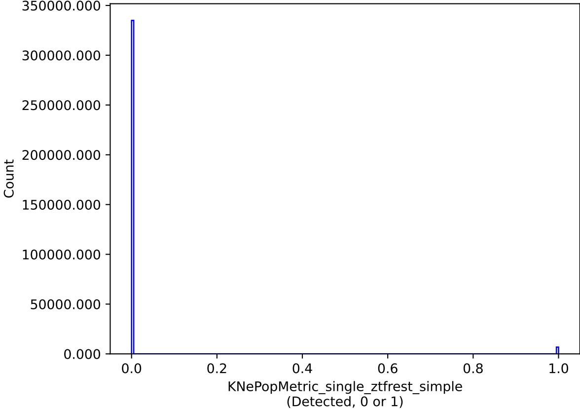
too_5_1v3.4_10yrs single model: KNePopMetric_single_ztfrest_simple
