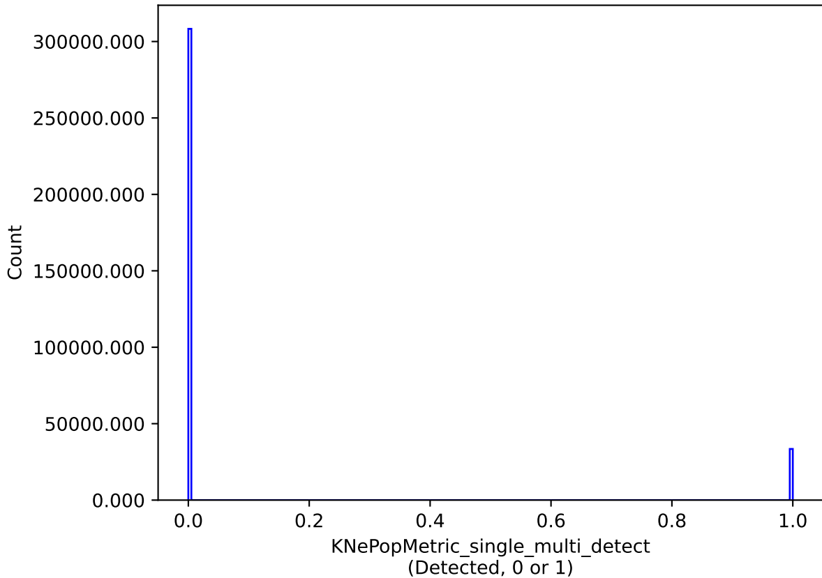
too_5_1v3.4_10yrs single model: KNePopMetric_single_multi_detect
