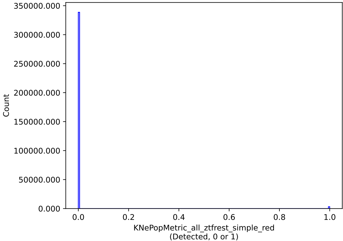
too_5_1v3.4_10yrs all models: KNePopMetric_all_ztfrest_simple_red
