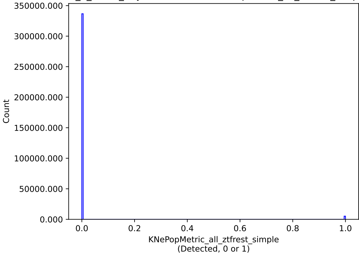
too_5_1v3.4_10yrs all models: KNePopMetric_all_ztfrest_simple
