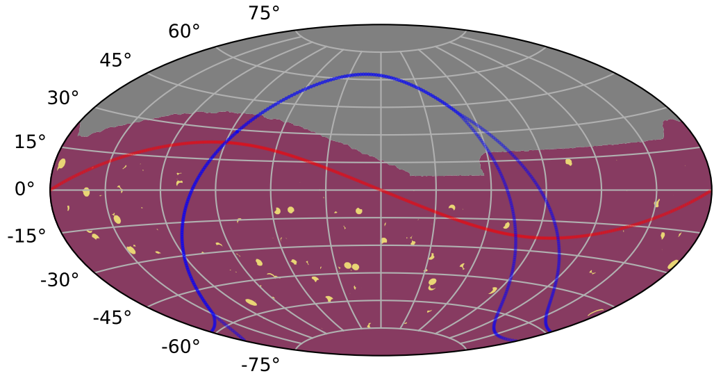
too_5_1v3.4_10yrs all models: KNePopMetric_all_red_color_detect
