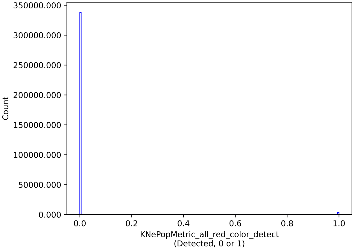
too_5_1v3.4_10yrs all models: KNePopMetric_all_red_color_detect
