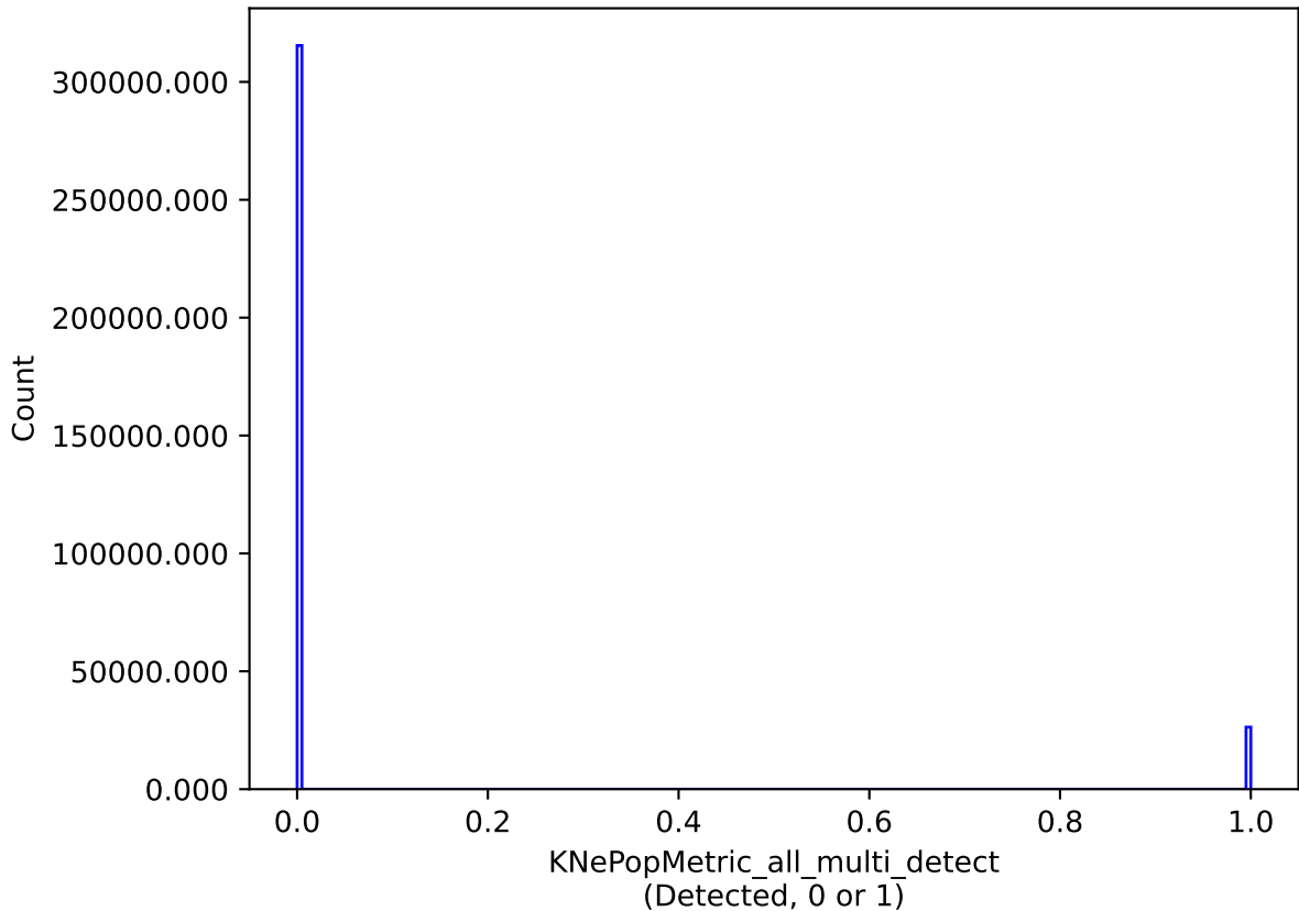
too_5_1v3.4_10yrs all models: KNePopMetric_all_multi_detect
