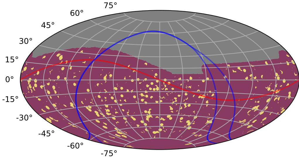
too_5_1v3.4_10yrs all models: KNePopMetric_all_multi_color_detect
