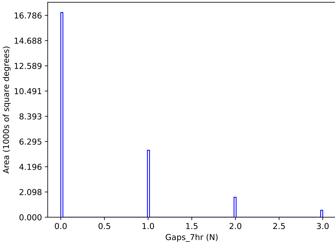
too_5_1v3.4_10yrs y band: Gaps_7hr
