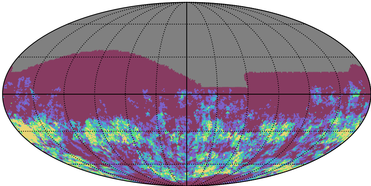
too_5_1v3.4_10yrs r band: Gaps_7hr
