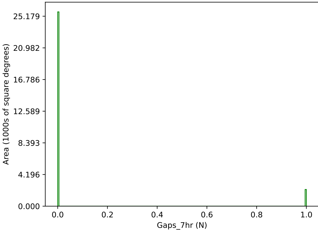
too_5_1v3.4_10yrs g band: Gaps_7hr
