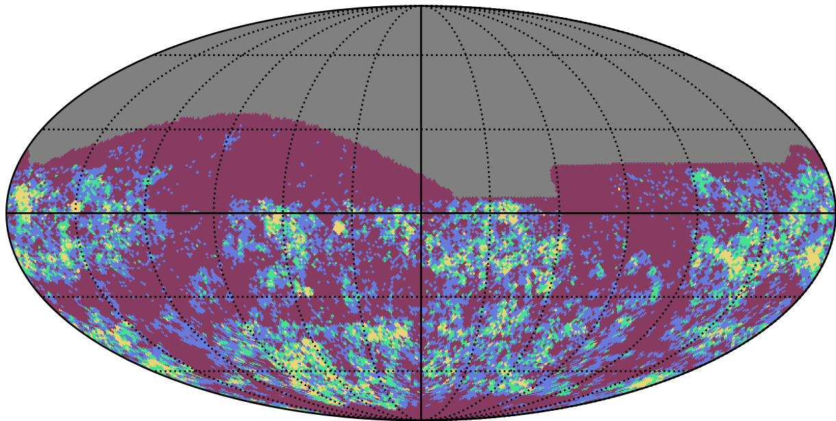
too_5_1v3.4_10yrs z band: Gaps_3hr
