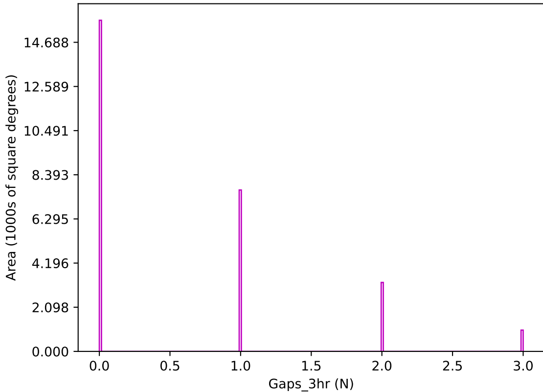
too_5_1v3.4_10yrs z band: Gaps_3hr
