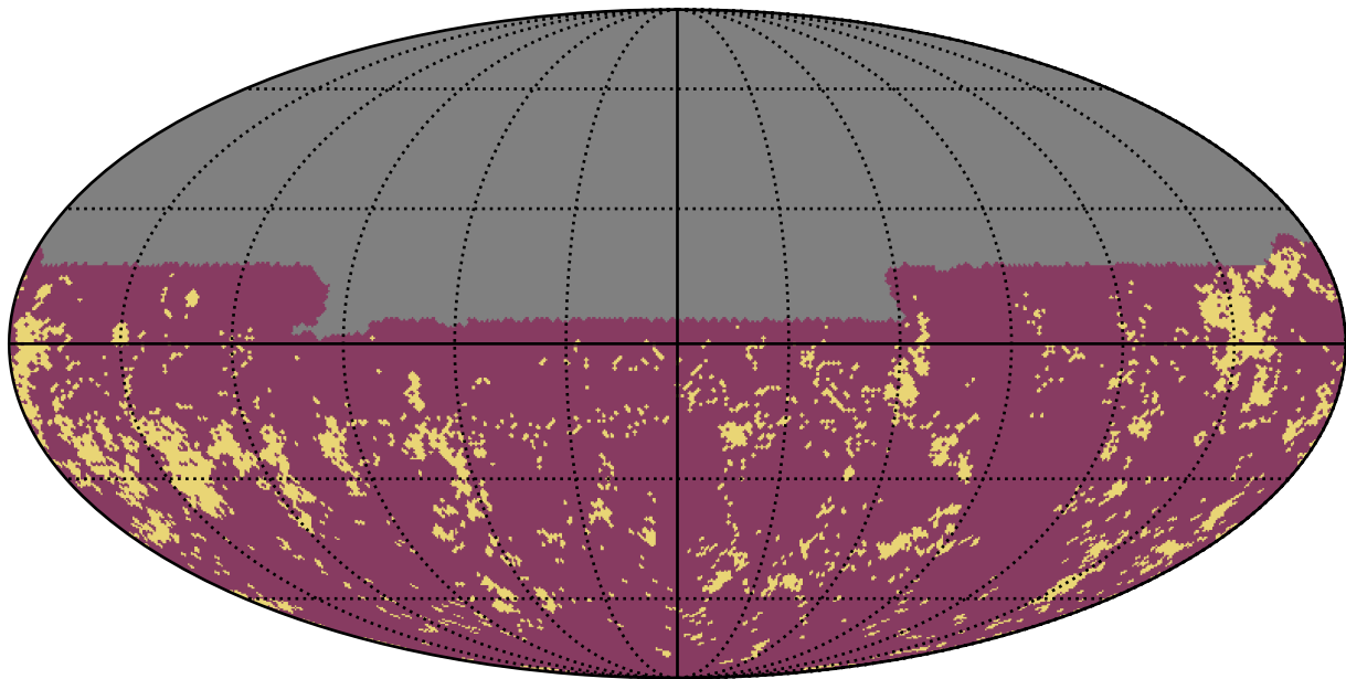
too_5_1v3.4_10yrs u band: Gaps_3hr
