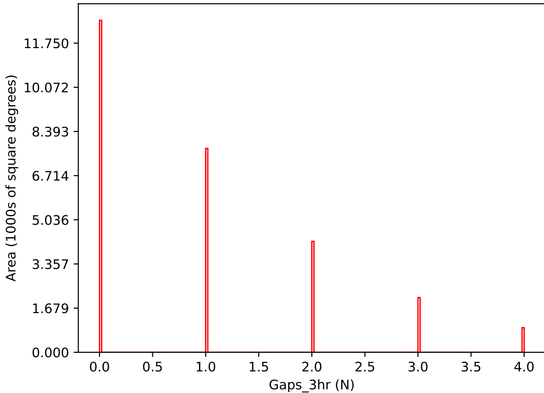
too_5_1v3.4_10yrs i band: Gaps_3hr
